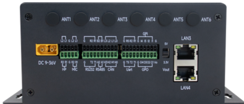
28F1E4 Backside interface indication diagram
